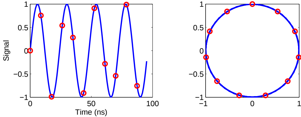
Figure 4: Sampling of the IF signal.
