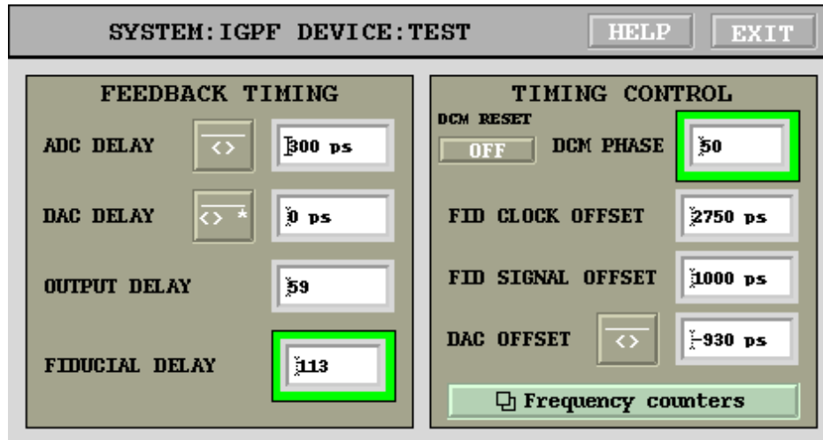
Figure 10: Timing panel
