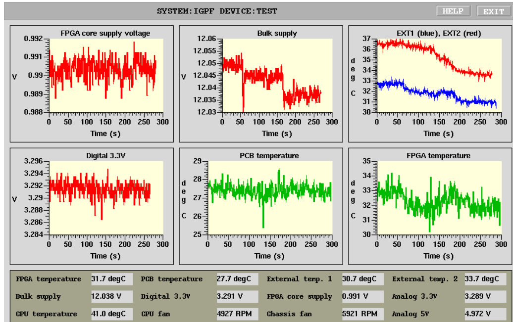
Figure 21: Environmental monitoring panel
