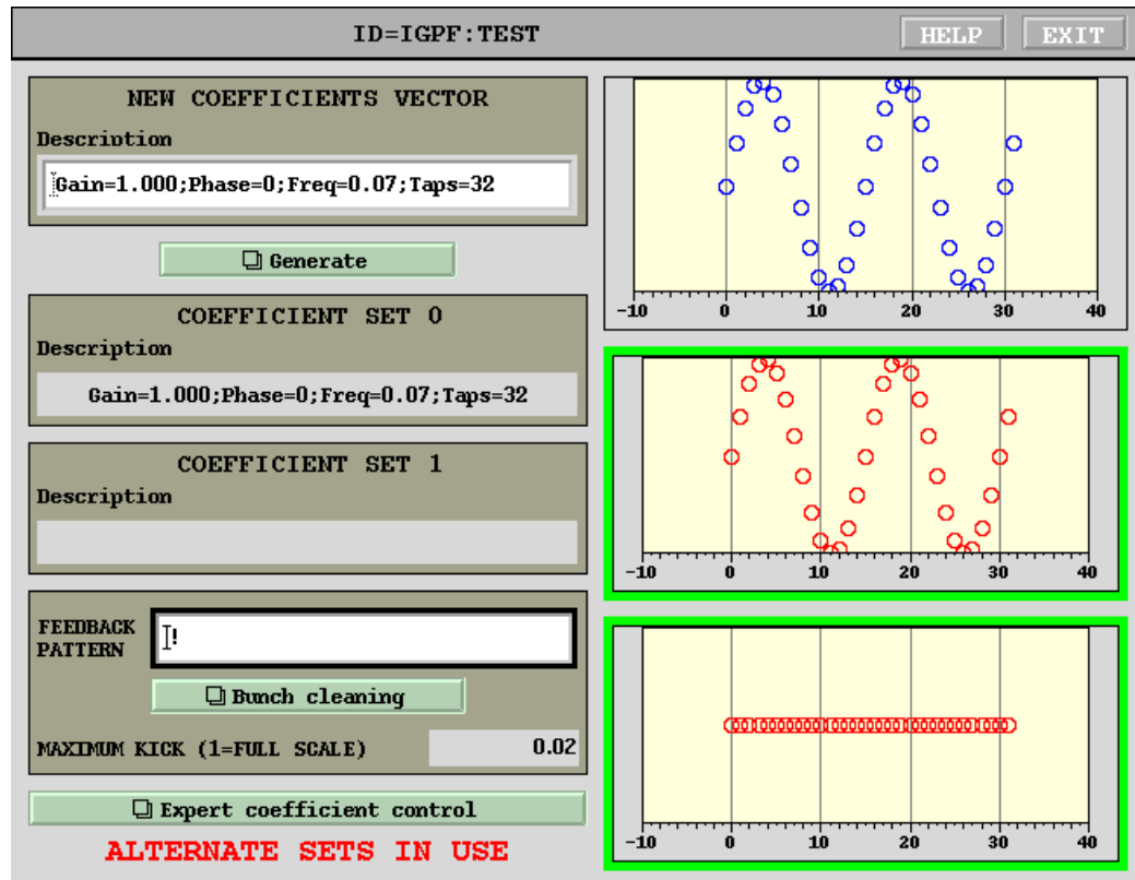
Figure 10: Coefficients panel
