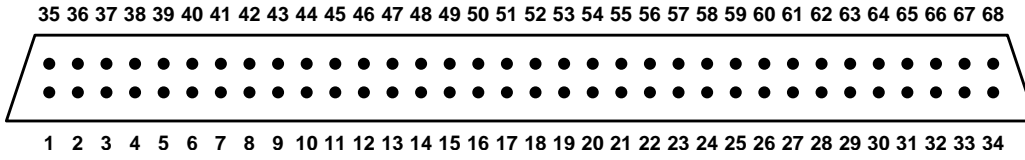
Figure 35: Pin numbering for general-purpose digital I/O connector
