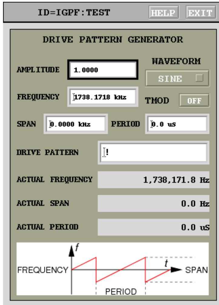
Figure 16: Drive panel
