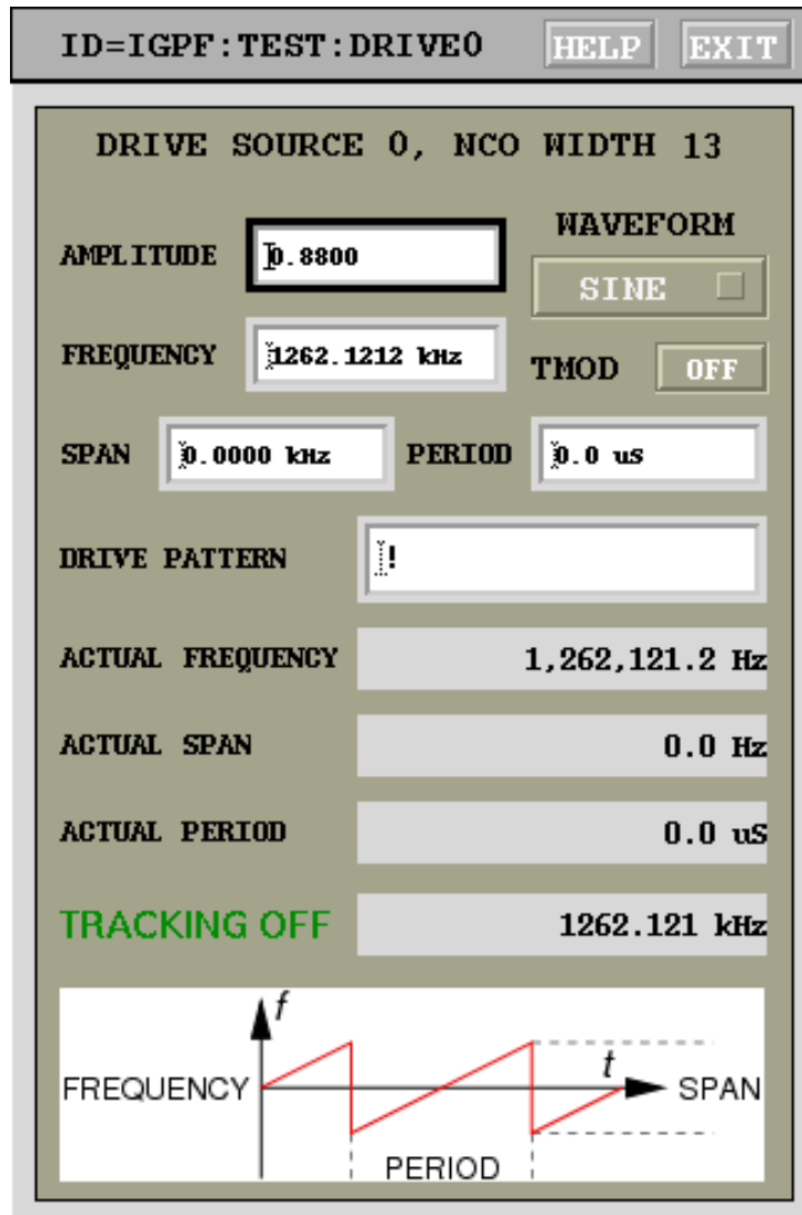
Figure 13: Drive panel
