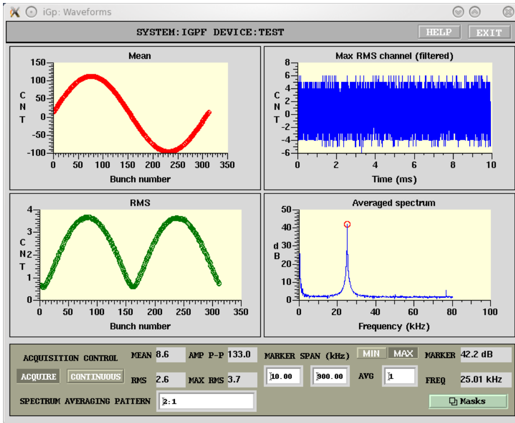
Figure 12: Waveforms panel
