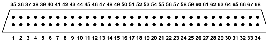
Figure 21: Pin numbering for general-purpose digital I/O connector
