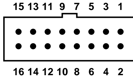
Figure 20: Pin numbering for 16-pin header-type front-panel connectors
